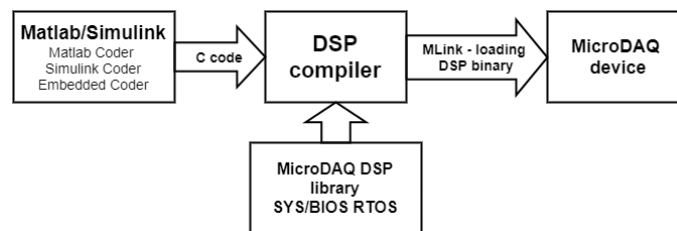
Figure 1 Software components
